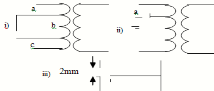
Figure 1: Fault classes i) Internal turn-to-turn fault, ii) Winding to ground fault, iii) Dielectric fault.
