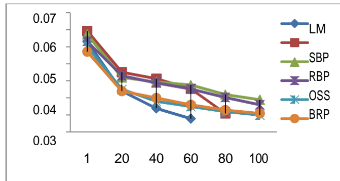
Figure 8: MAPE for different algorithms in case of winding to ground fault
