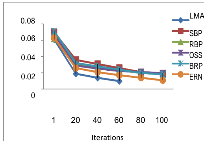
Figure.6: MAPE for different algorithms in case of dielectric fault
