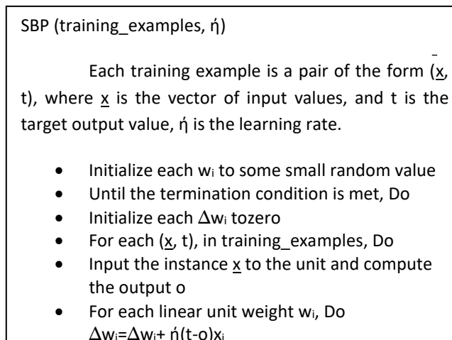
Figure. 4: Weight updates process of a generalized SBP
