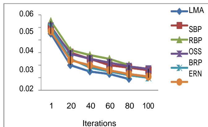
Figure7: MAPE for different algorithms in case of inter-turn fault
